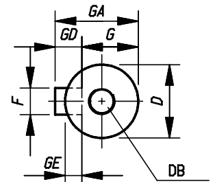
SHAFT
